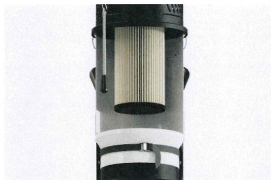
Bottomless cartridge filter for perfect dust discharge
